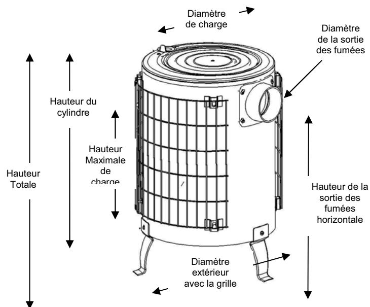
Figure 1: dimensions
